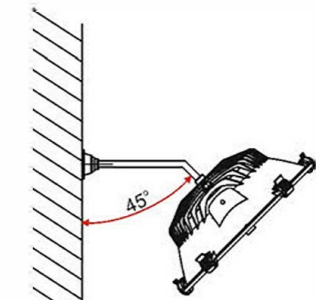
Wall mounting
